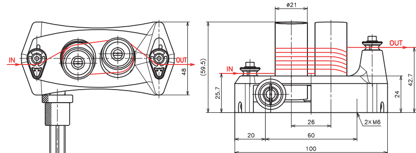
図面=D510059-R
